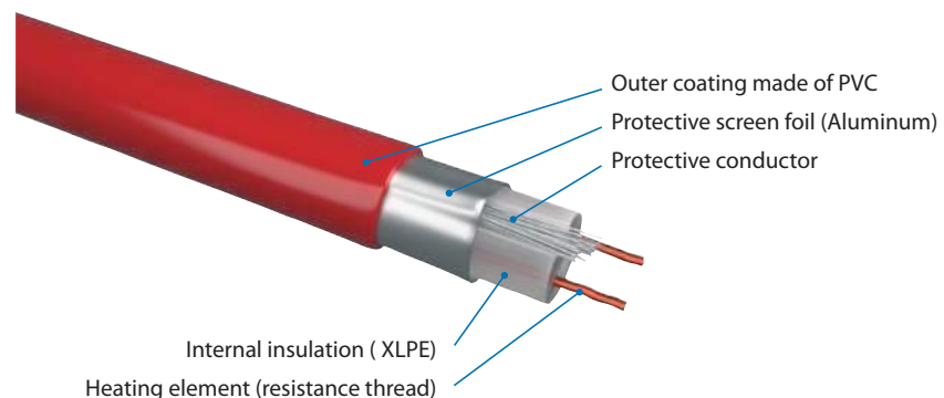
DEVIflex™ heating cable construction
