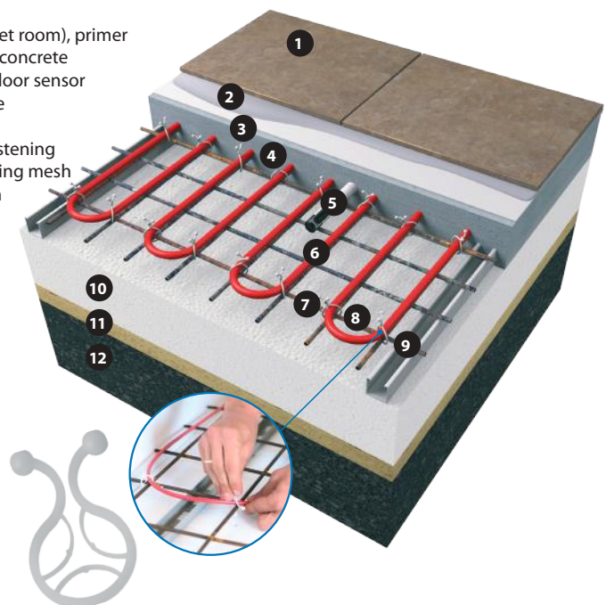
Fig. 5. Cable heating in concrete with cable fixed to reinforcement mesh by DEVclip™ Twist.
