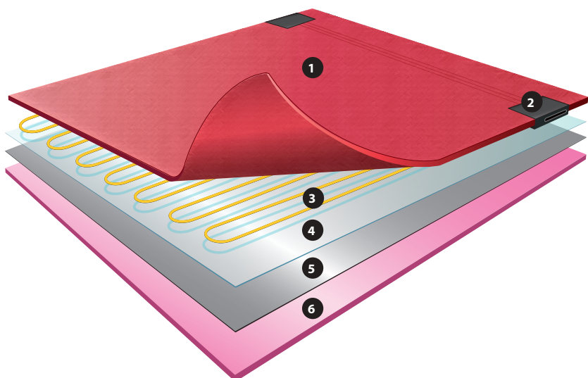
Fig. 15. DEVDry™ heating element construction
