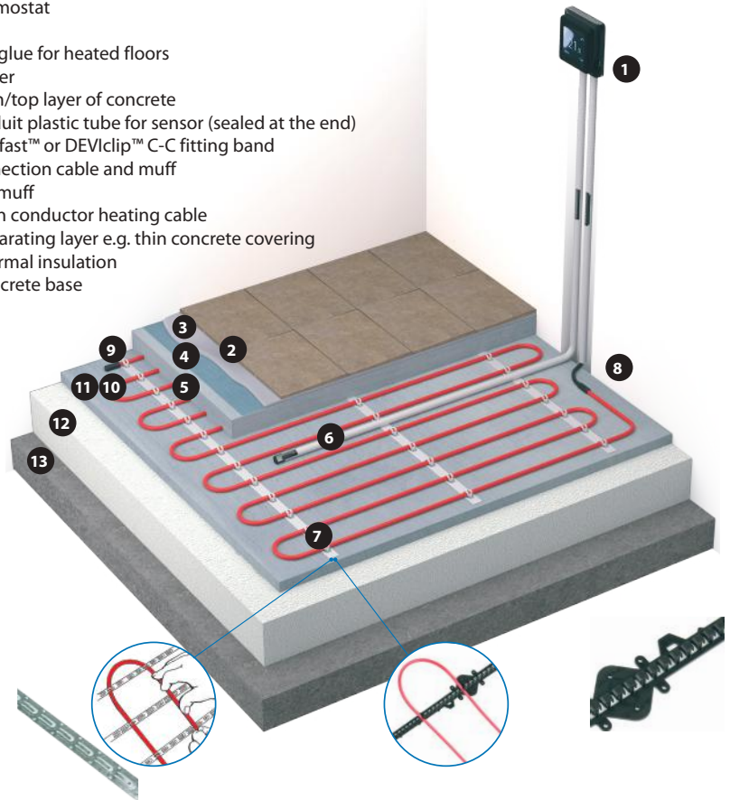
Fig. 4. Cable heating in concrete floor with cable fixed by DEVIfast™ or DEVclip™ C-C fitting band.
