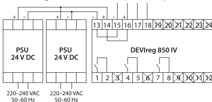
**Fig. H — connection of 2 pcs. PSU in parallel
